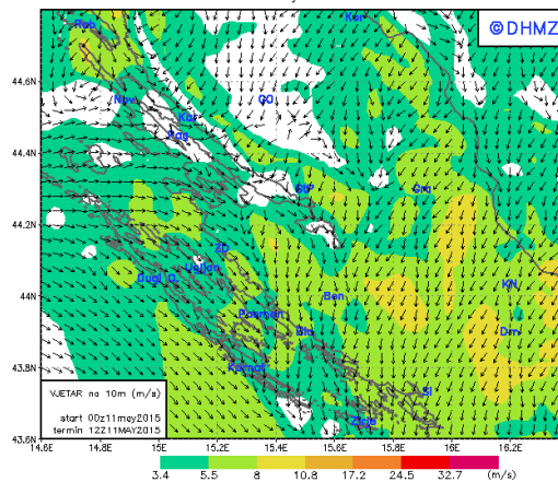
DAda MASLENICA 10m vjetar u 12 UTC 11MAY2015
